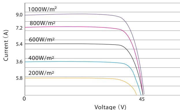
Current-Voltage Characteristic (I-V Curve)
