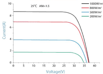
IV-CURVES of PV module RD310M6
