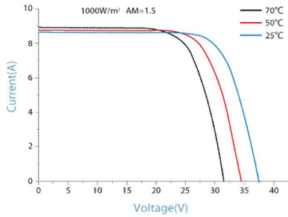
IV-CURVES of PV module RD310M6
