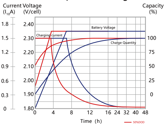
Constant-potential charge
