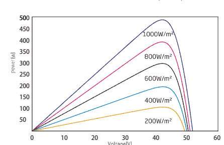
P-V Curve at Different Irradiation (490W)
