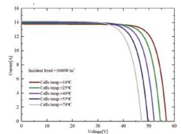
I-V Curves of SSD590AHJH at different cell temperature
