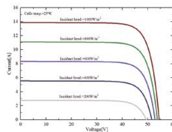
I-V Curves of SSD590AHJH at different irradiance
