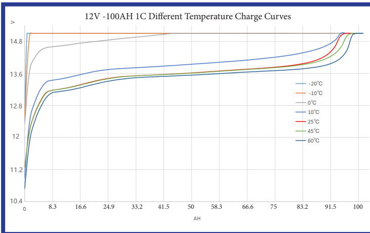
Charging rates at different temperatures.
