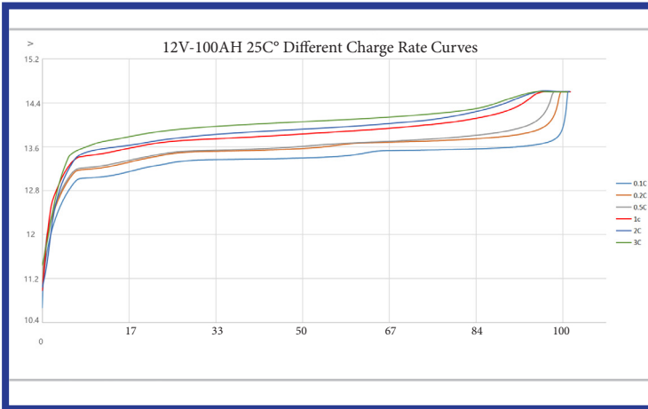
Charging rate at different amps.
