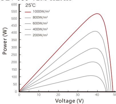
Power curve under different irradiance OLV-535-72M-HEAH
