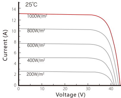
I-V Curves at Different Irradiances OLV-535-72M-HEAH
