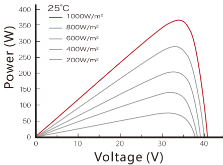
Power curve under different irradiance OLV-365-60M-HC9H
