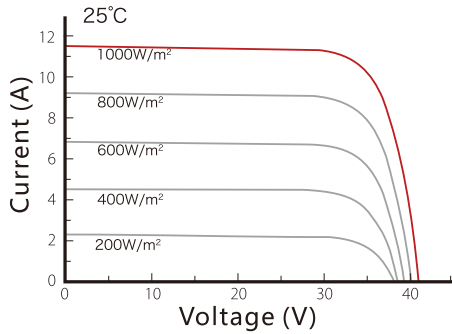
I-V Curves at Different Irradiances OLV-365-60M-HC9H
