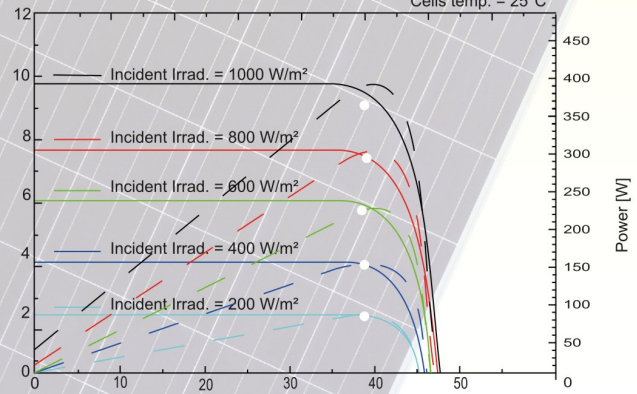
Current-Voltage & Power-Voltage Curve Cells temp. = 25°C
