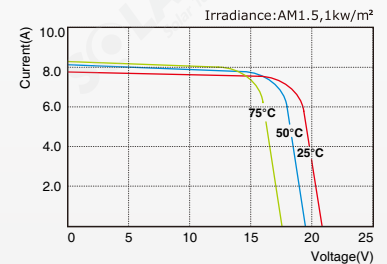
SLP130-12U I-V Curves
