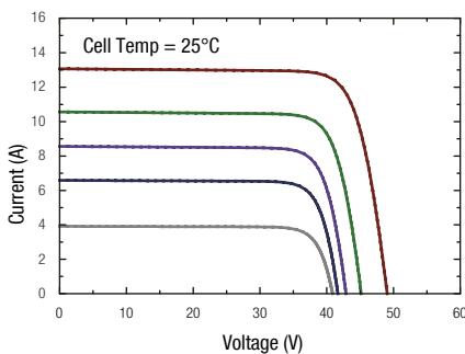
Current-Voltage and Power-Voltage Curves
