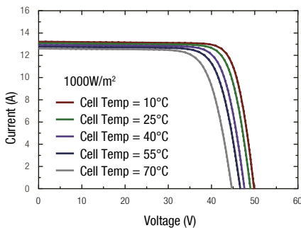
Temperature Dependence of Isc, Voc, Pmax
