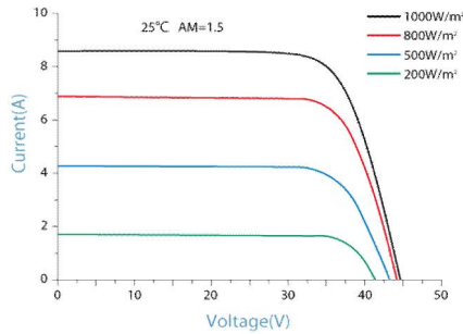
IV-CURVES of PV module RD330P6
