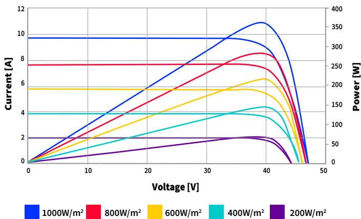
Current-Voltage & Power-Voltage Curve (360)
