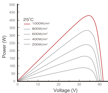
Power curve under different irradiance OLV-445-60M-DEAH
