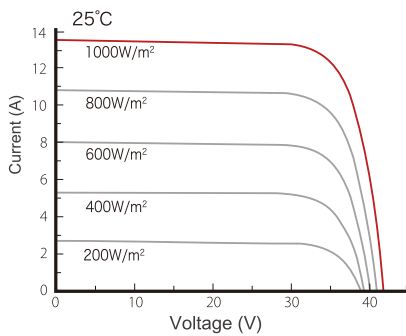
I-V Curves at Different Irradiances OLV-445-60M-DEAH
