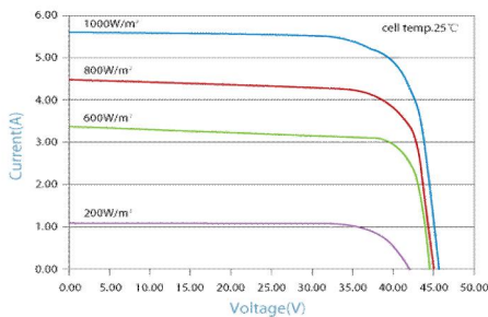
IV-CURVES of PV module RD190M5
