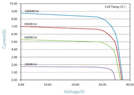
IV-CURVES of PV module RD260P6
