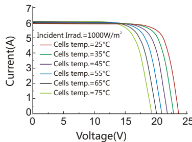
Current-Voltage Curve
