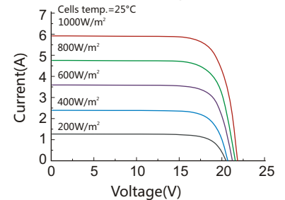
Current-Voltage Curve
