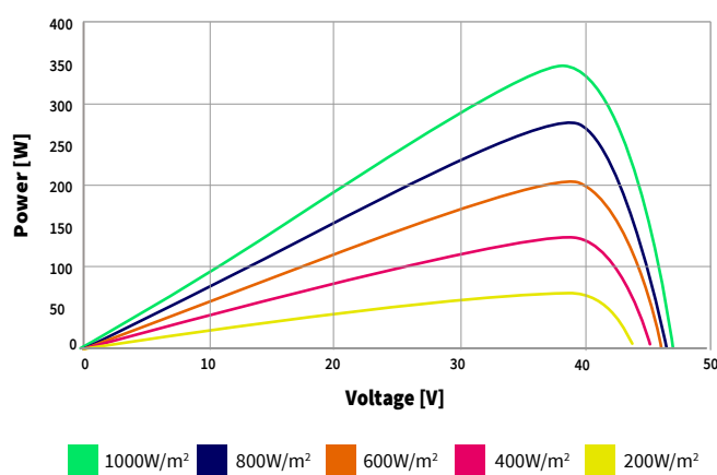
Power-Voltage Curve (345 W)
