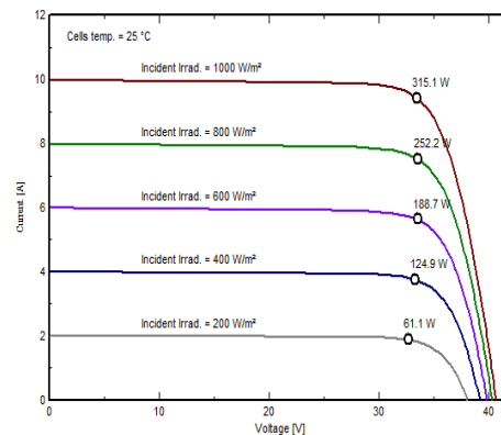
I-V Curve of 315W at 25°C cell temp. and different Irradiance level
