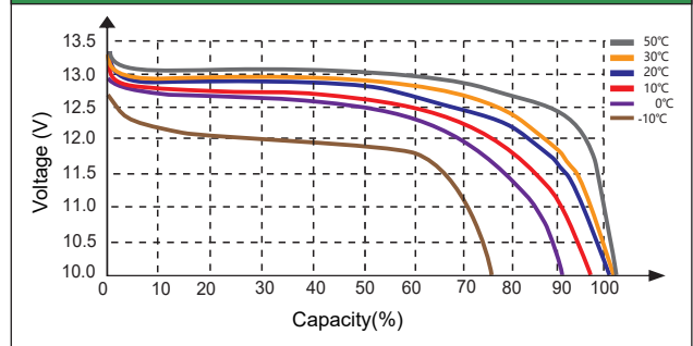
DIFFERENT TEMPERATURE DISCHARGE CURVE (0.5C)
