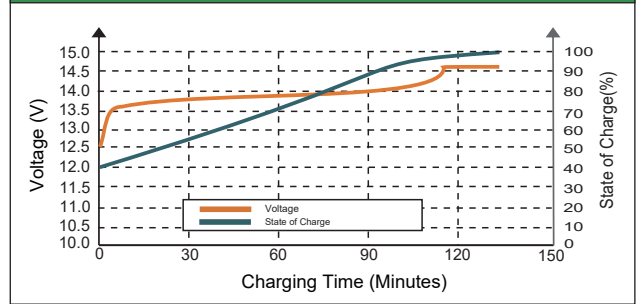
STATE OF CHARGE CURVE (0.5C, 25°C)
