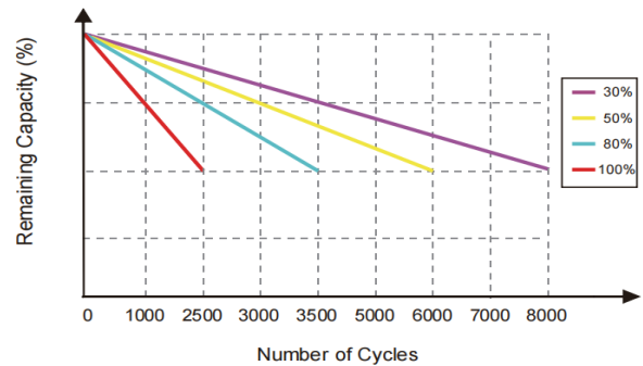
CYCLE LIFE vs. DEPTH OF DISCHARGE(DOD)
