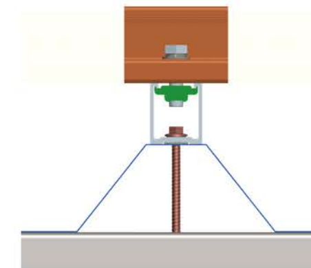
① Connection of clamp and Rail
