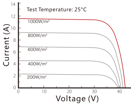
I-V Curves at Different Irradiances OLV-440-72M-HC6H
